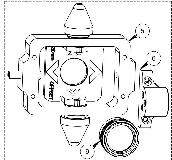
5910-01-050-XXX YOKE ASSY, MINI PRISM, SIDE VIAL, 0/30
